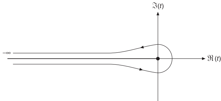
FIGURE 14.5 Contour, Schlaefli integral for J_\nu .
