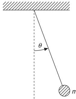
FIGURE 22.9 Simple pendulum.
