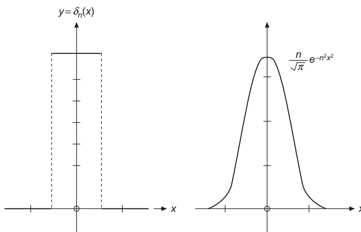
FIGURE 1.21 \delta -Sequence function: left, Eq. (1.152); right, Eq. (1.153).
