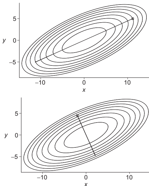
FIGURE 6.2 Trajectories starting at rest. Top: At a point on the line x = y\sqrt{5} . Bottom: At a point on the line y = -x\sqrt{5} .
