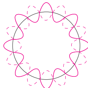
Circumference = 8 wavelengths
