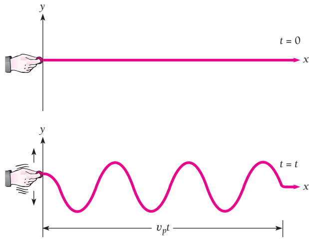
Figure 3.2 Wave propagation.
