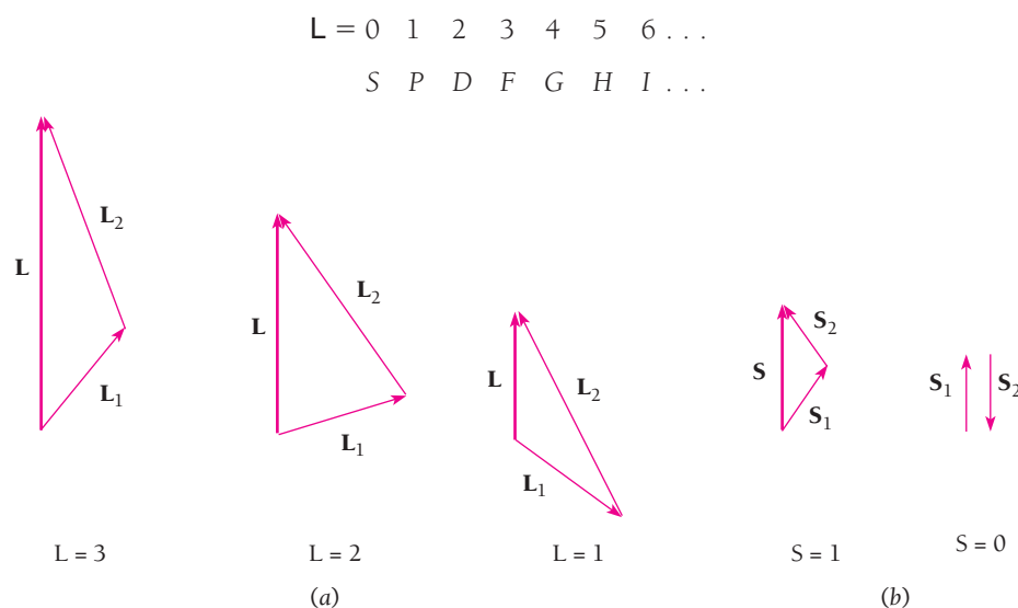
Figure 7.19 When l_1 = 1 , s_1 = \frac{1}{2} , and l_2 = 2 , s_2 = \frac{1}{2} , there are three ways in which \mathbf{L}_1 and \mathbf{L}_2 can combine to form \mathbf{L} and two ways in which \mathbf{S}_1 and \mathbf{S}_2 can combine to form \mathbf{S} .
