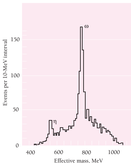
Figure 13.4 Resonant states in the reaction \pi^+ + p \rightarrow \pi^+ + p + \pi^+ + \pi^- + \pi^0 occur at effective masses of 549 and 783 \text{MeV}/c^2 . By effective mass is meant the total energy, including mass energy, of the three new mesons relative to their center of mass.
