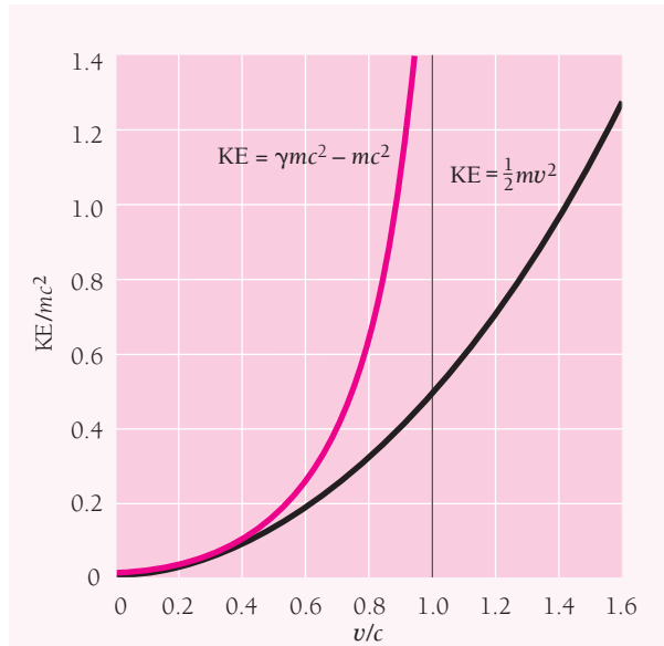
Figure 1.16 A comparison between the classical and relativistic formulas for the ratio between kinetic energy \text{KE} of a moving body and its rest energy mc^2 . At low speeds the two formulas give the same result, but they diverge at speeds approaching that of light. According to relativistic mechanics, a body would need an infinite kinetic energy to travel with the speed of light, whereas in classical mechanics it would need only a kinetic energy of half its rest energy to have this speed.
