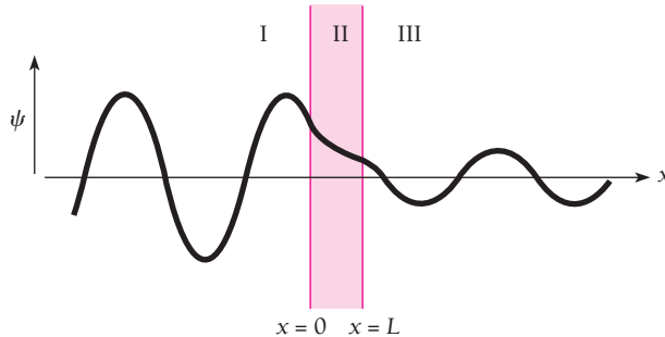
Figure 5.14 At each wall of the barrier, the wave functions inside and outside it must match up perfectly, which means that they must have the same values and slopes there.
