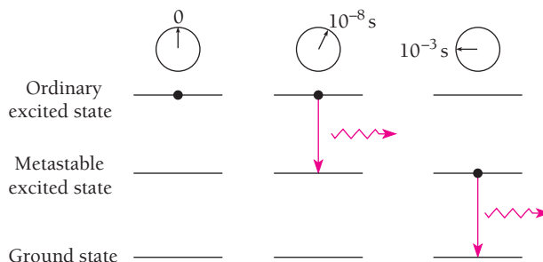
Figure 4.24 An atom can exist in a metastable energy level for a longer time before radiating than it can in an ordinary energy level.
