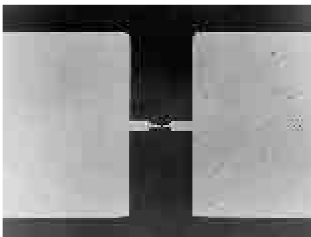
The small rectangle at the center of this photograph is a Josephson junction 1.25 \mu\text{m} wide.
