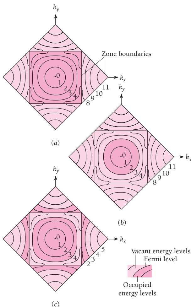
Figure 10.48 Electron energy contours and Fermi levels in three types of solid: (a) insulator; (b) monovalent metal; (c) divalent metal. Energies are in electronvolts.
