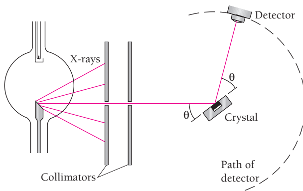
Figure 2.21 X-ray spectrometer.
