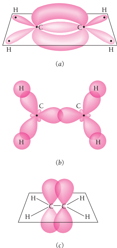
Figure 8.14 (a) The ethylene ( \text{C}_2\text{H}_4 ) molecule. All the atoms lie in a plane perpendicular to the plane of the paper. (b) Top view, showing the sp^2 hybrid orbitals that form \sigma bonds between the C atoms and between each C atoms. (c) Side view, showing the pure p_x orbitals that form a \pi bond between the C atoms.
