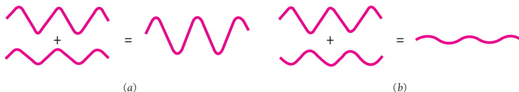
Figure 2.3 (a) In constructive interference, superposed waves in phase reinforce each other. (b) In destructive interference, waves out of phase partially or completely cancel each other.
