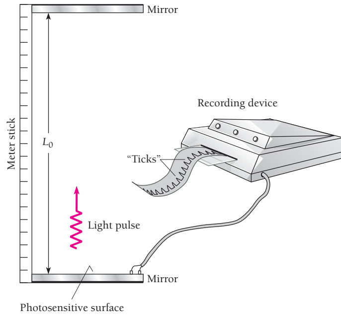
Figure 1.3 A simple clock. Each “tick” corresponds to a round trip of the light pulse from the lower mirror to the upper one and back.
