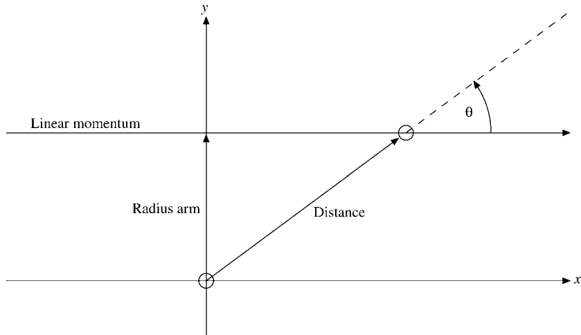
FIGURE 1.12 Angular momentum.
