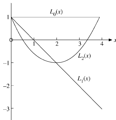
FIGURE 13.4 Laguerre polynomials.
