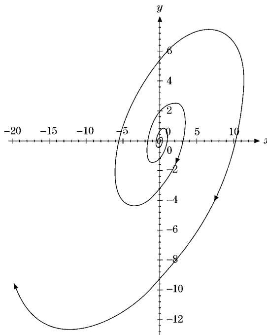
FIGURE 18.9 Spiral point.
