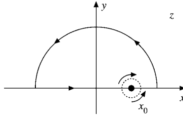
FIGURE 7.3 Closing the contour with an infinite-radius semicircle.
