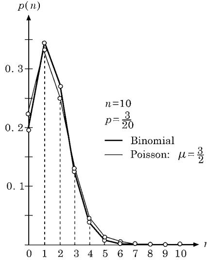
FIGURE 19.6 Poisson distribution compared with binomial distribution.
