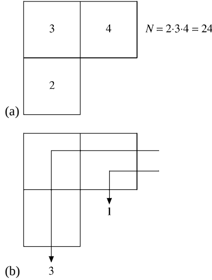
FIGURE 4.9 Illustration of (a) N and (b) D in Eq. (4.125) for the octet Young tableau of SU(3) .
