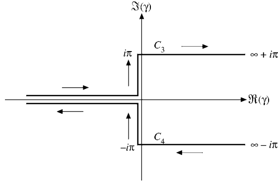
FIGURE 11.9 Hankel function contours.
