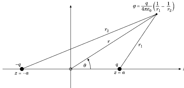
FIGURE 12.3 Electric dipole.
