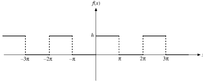
FIGURE 14.5 Square wave.
