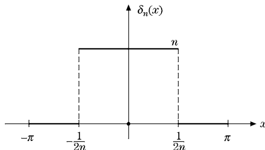
FIGURE 14.9 Rectangular pulse.
