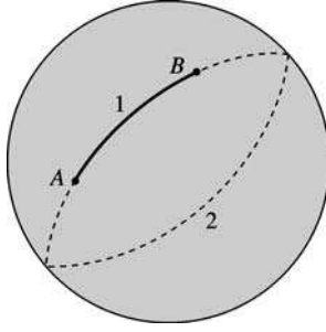
FIGURE 17.2 Stationary paths over a sphere.
