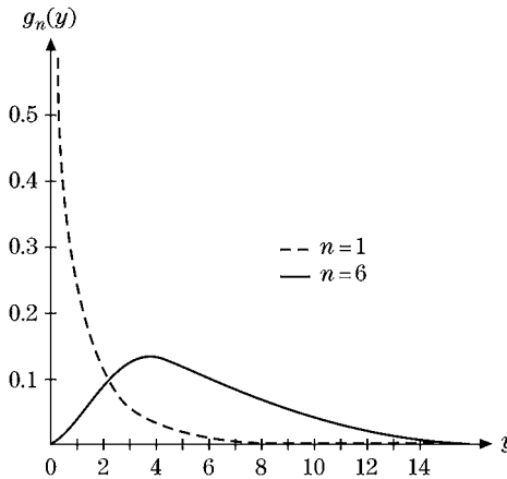
FIGURE 19.11 \chi^2 probability density g_n(y) .
