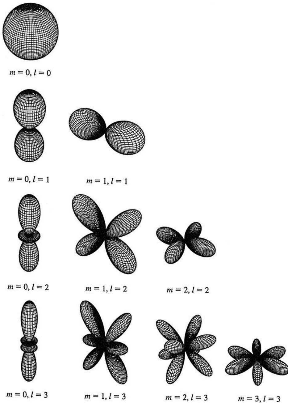
FIGURE 12.15 [Y_l^m(\theta, \varphi)]^2 for 0 \leq l \leq 3, m = 0, \dots, 3 .
