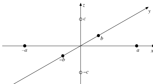
FIGURE 4.12 D_2 symmetry.
