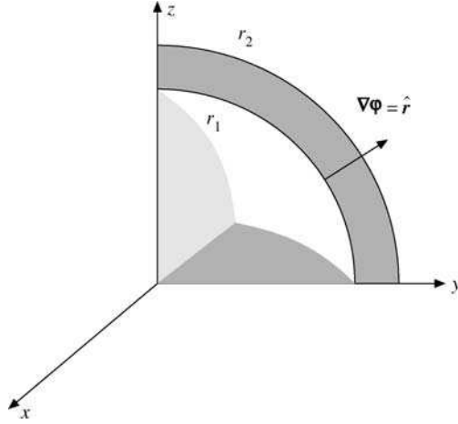
FIGURE 1.21 Gradient for \varphi(x, y, z) = (x^2 + y^2 + z^2)^{1/2} , spherical shells: (x_2^2 + y_2^2 + z_2^2)^{1/2} = r_2 = C_2 , (x_1^2 + y_1^2 + z_1^2)^{1/2} = r_1 = C_1 .
