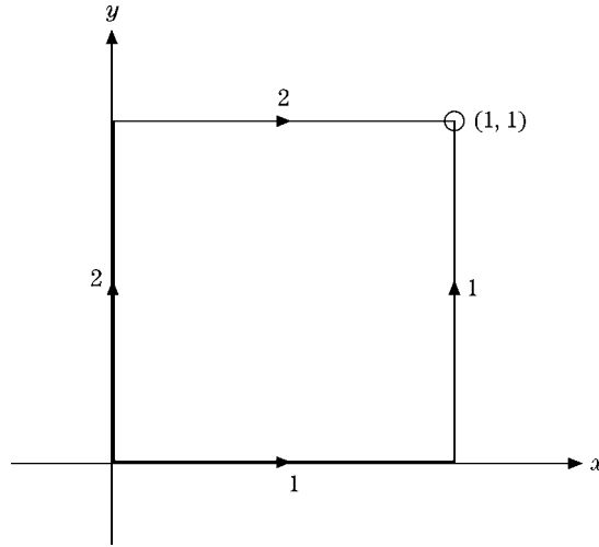
FIGURE 6.10 Contour.
