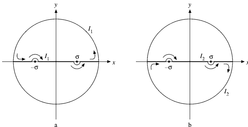
FIGURE 7.8 Contours.
