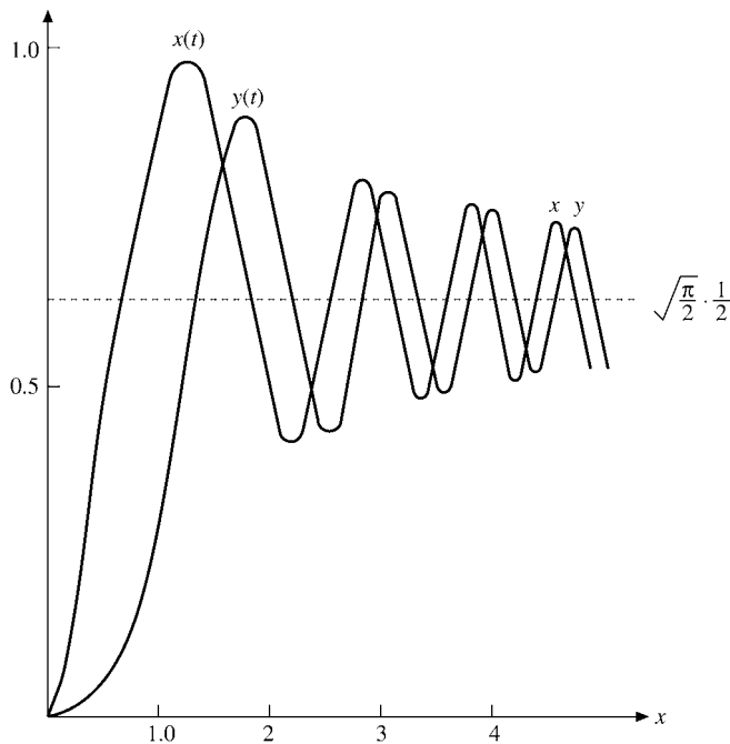
FIGURE 11.15 Fresnel integrals.
