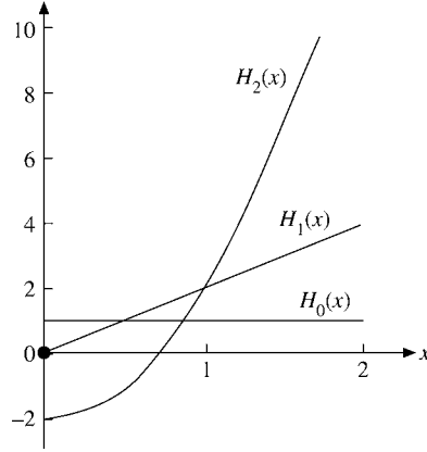
FIGURE 13.1 Hermite polynomials.
