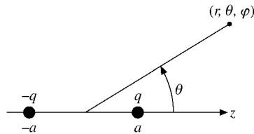
FIGURE 12.14 Electric dipole.
