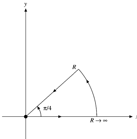
FIGURE 7.15 Angle contour.
