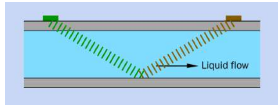
Figure 16-7 Some ultrasound flow sensors are designed to be clamped externally to a pipe.
