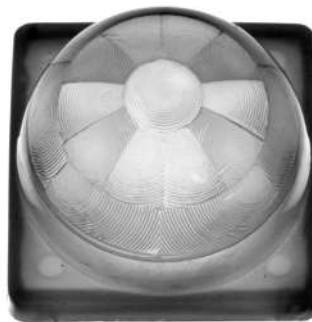
Figure 4-9 A mosaic weighted more toward sensing lateral motion. The grooves of the fresnel lenses are visible.
